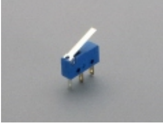
33156 pilot switch for lid position 1 N / 1 NC : 250 V AC / 5 A; 30 V DC / 4 A
